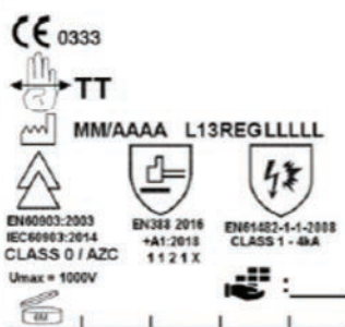
Marking example
